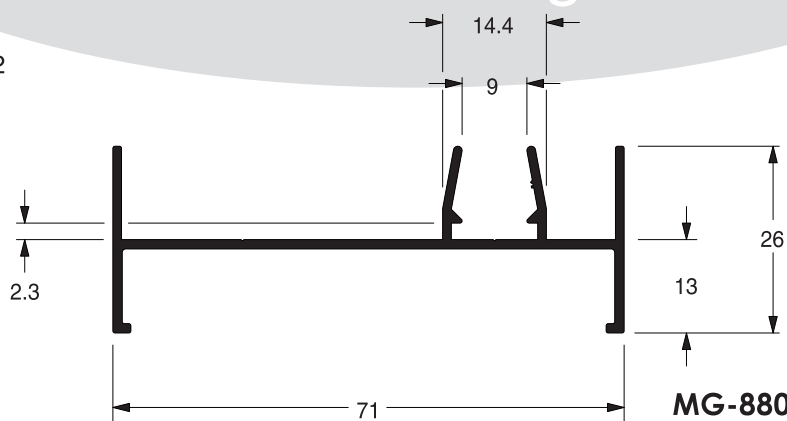
Marco lateral / correr 2
