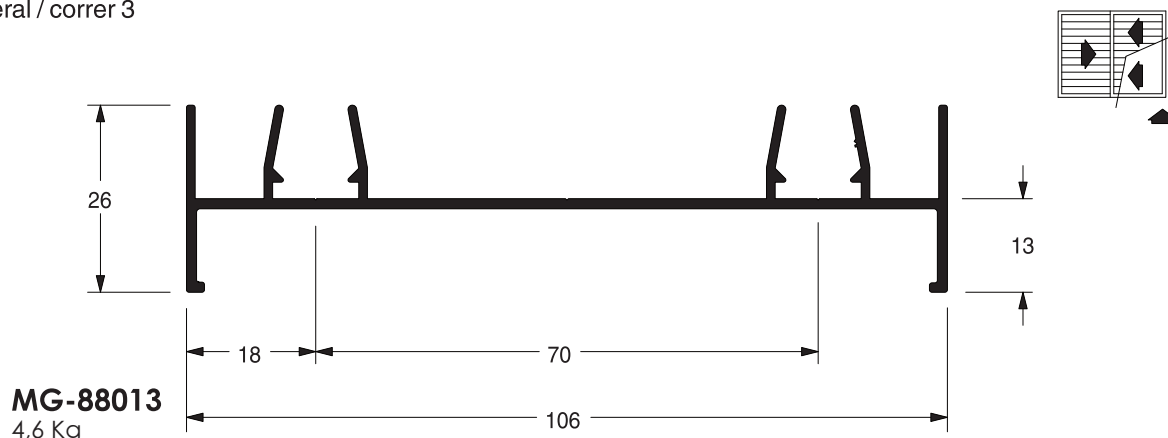
Marco lateral / correr 3
